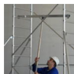
The braces and midbraces are easily put in place using the T-Grip pole
