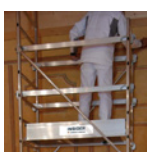
Braces equipped with notched jaws that lock on the rungs
